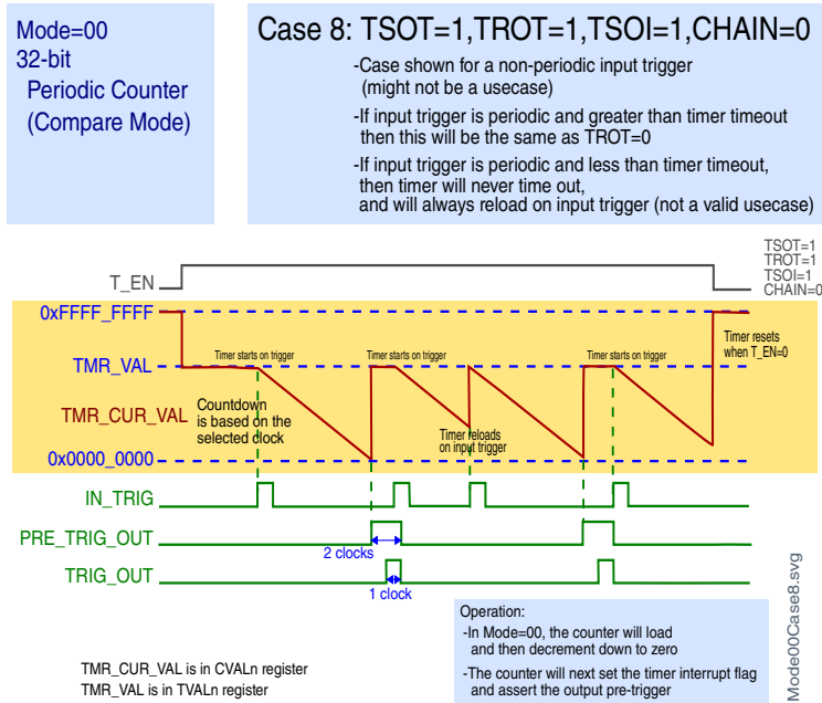
Figure 48-12. Case 8: TSOT = 1, TROT = 1, TSOI = 1, CHAIN = 0
