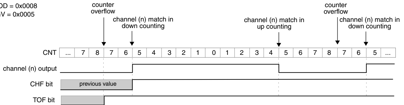
Figure 47-28. CPWM signal with ELSB:ELSA = 1:0
