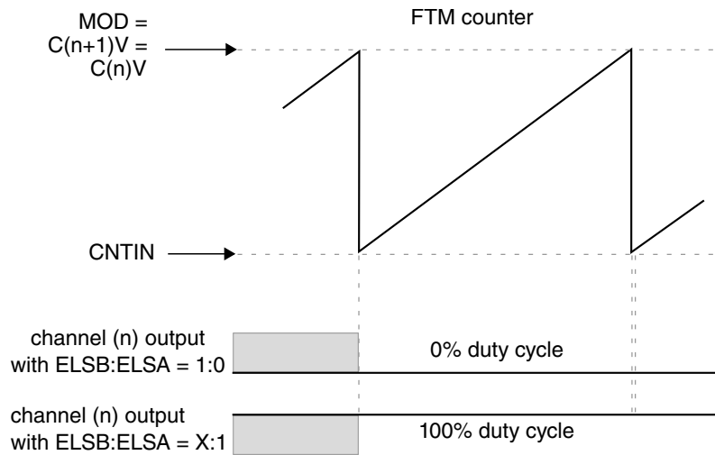
Figure 47-39. Channel (n) output if (C(n)V = C(n+1)V = MOD)
