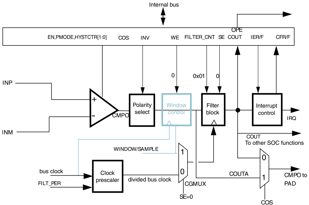
Figure 45-6. Sampled, Non-Filtered (# 3B): sampling interval internally derived
