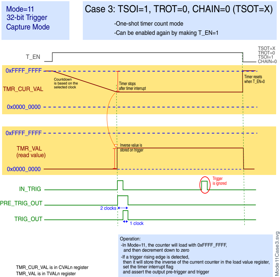
Figure 48-18. Case 3: TSOT = X, TROT = 0, TSOI = 1, CHAIN = 0
