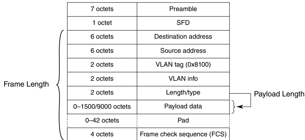
Figure 57-3. VLAN-tagged MAC frame format overview
