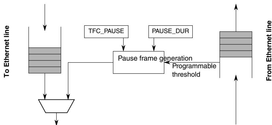
Figure 57-8. Pause frame generation overview
