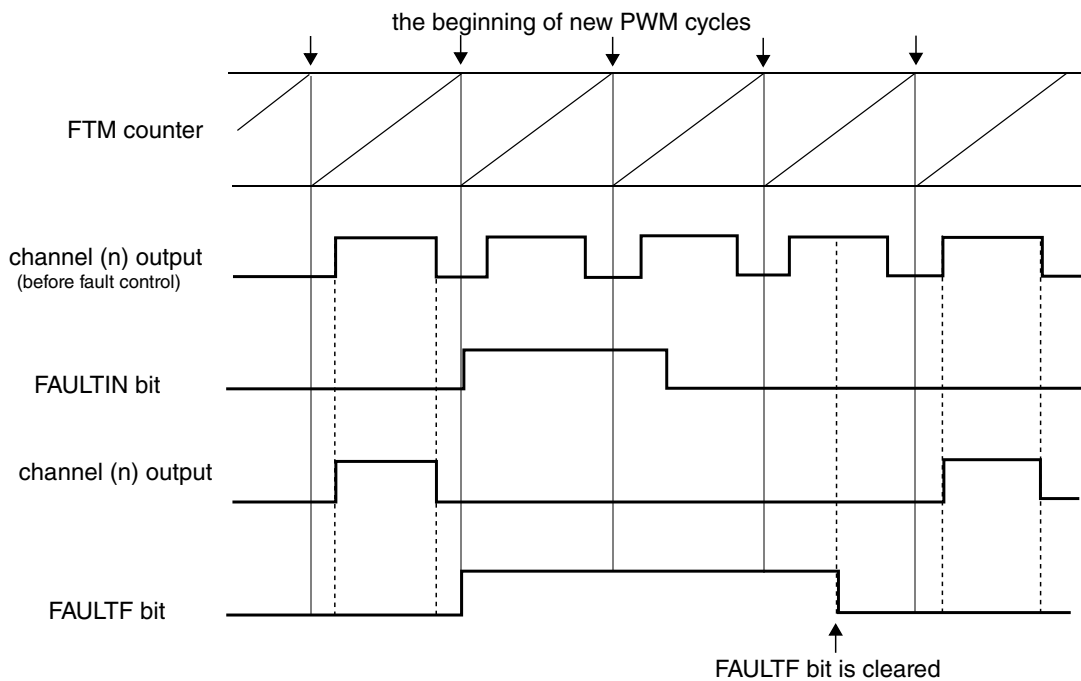
Figure 47-85. Fault control with manual fault clearing
