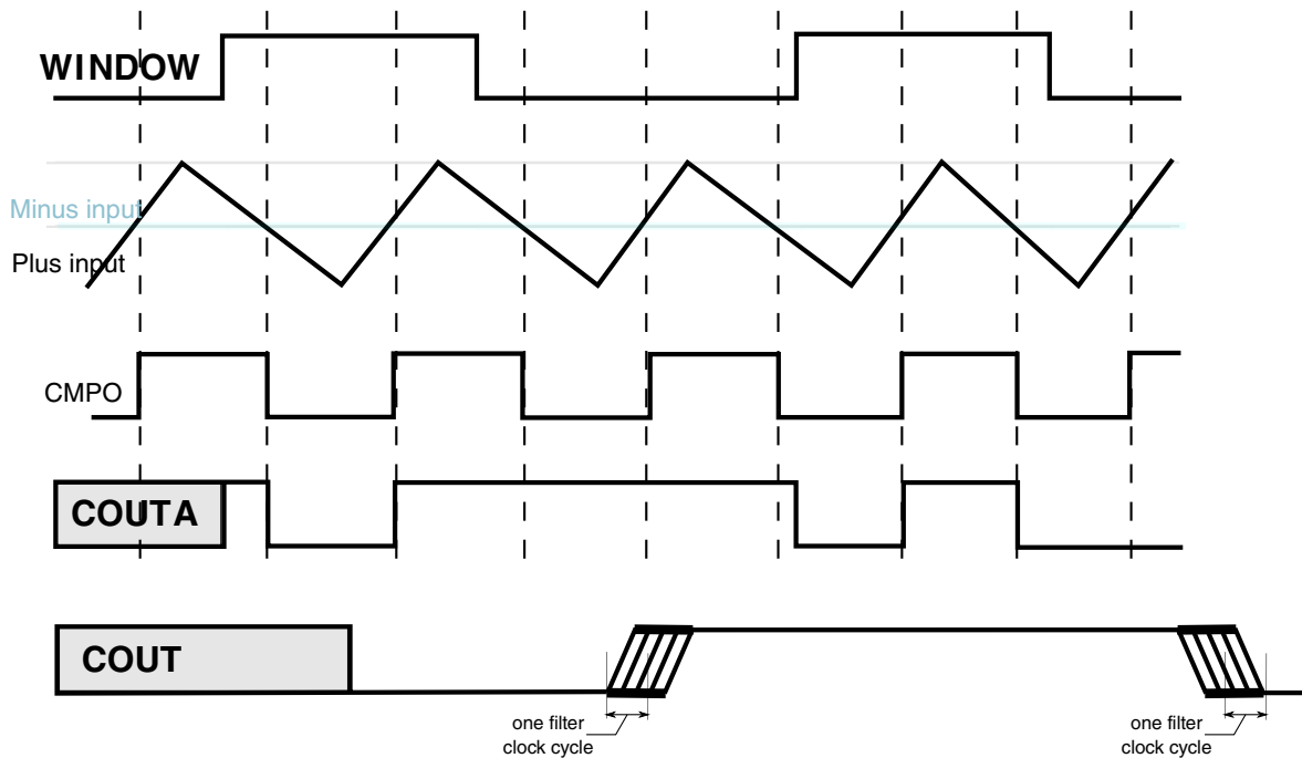
Figure 45-14. Windowed/Filtered mode operation
