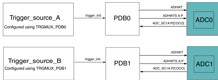
Figure 43-3. ADCs triggering with independent sources
