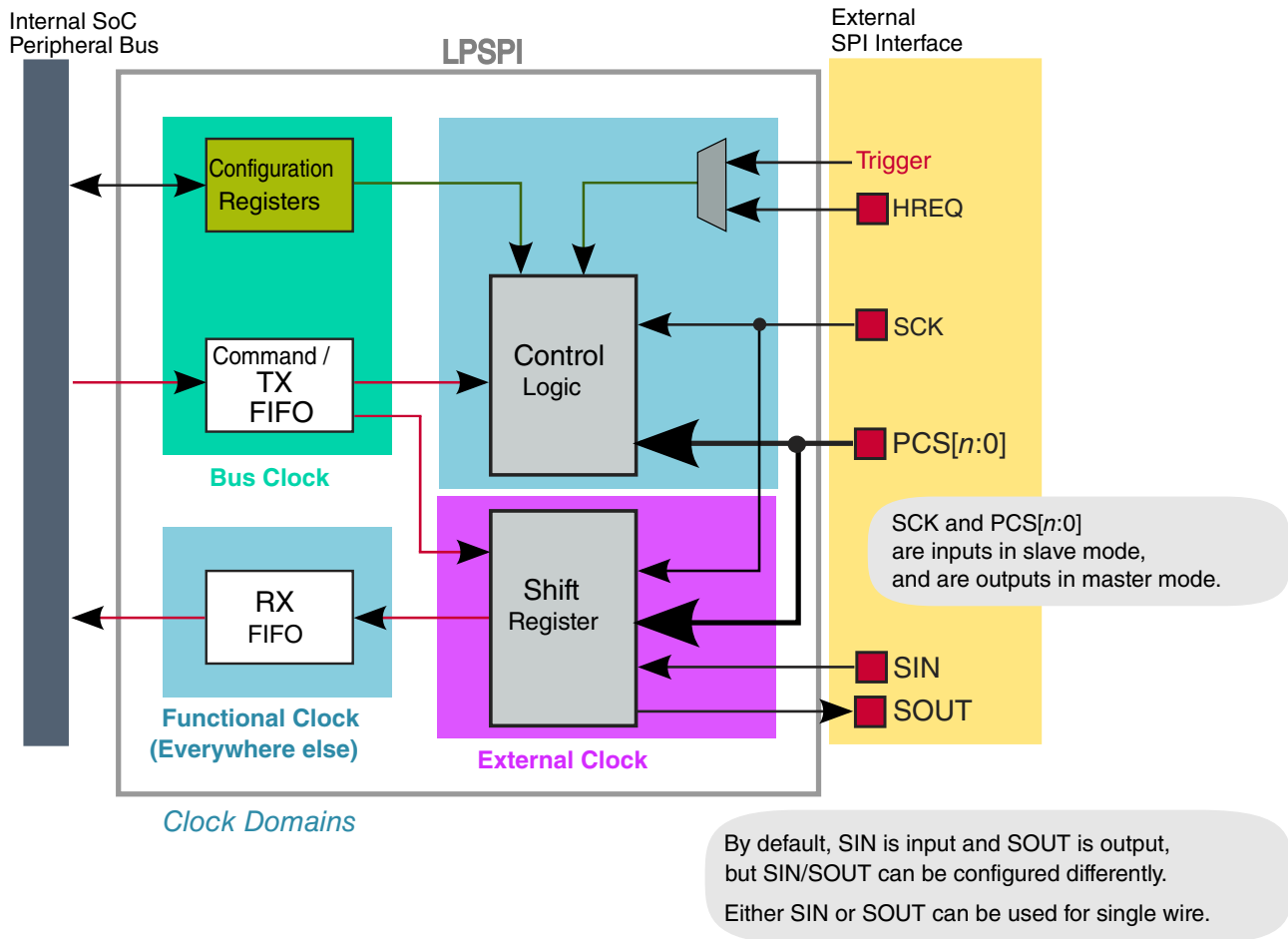
Figure 51-1. Block Diagram
