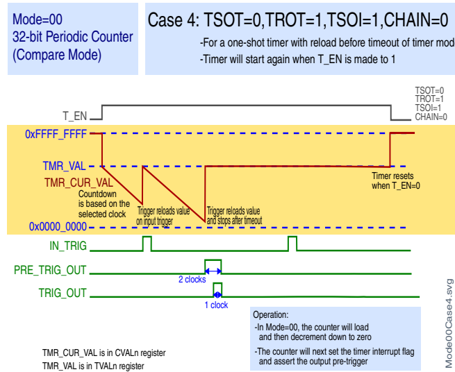
Figure 48-8. Case 4: TSOT = 0, TROT = 1, TSOI = 1, CHAIN = 0
