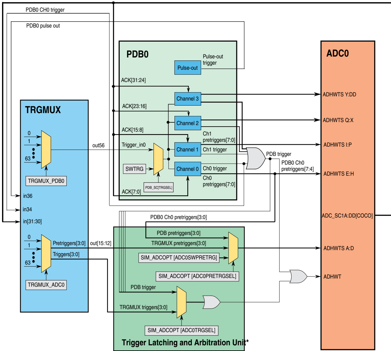
Figure 43-2. ADC0_PDB0 ADC Triggering scheme example
