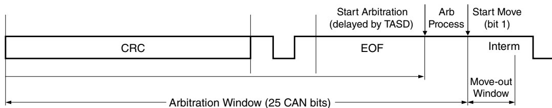
Figure 55-13. Arbitration and move-out time windows
