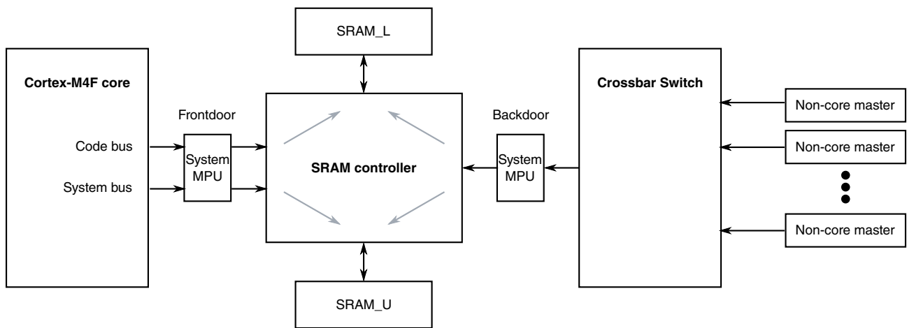
Figure 31-1. SRAM accessibility
