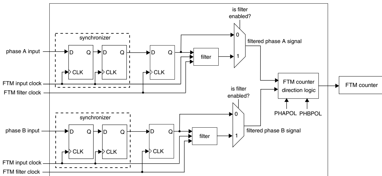
Figure 47-102. Diagram for Quadrature Decoder when FLTIPS[3:0] ≠ 0
