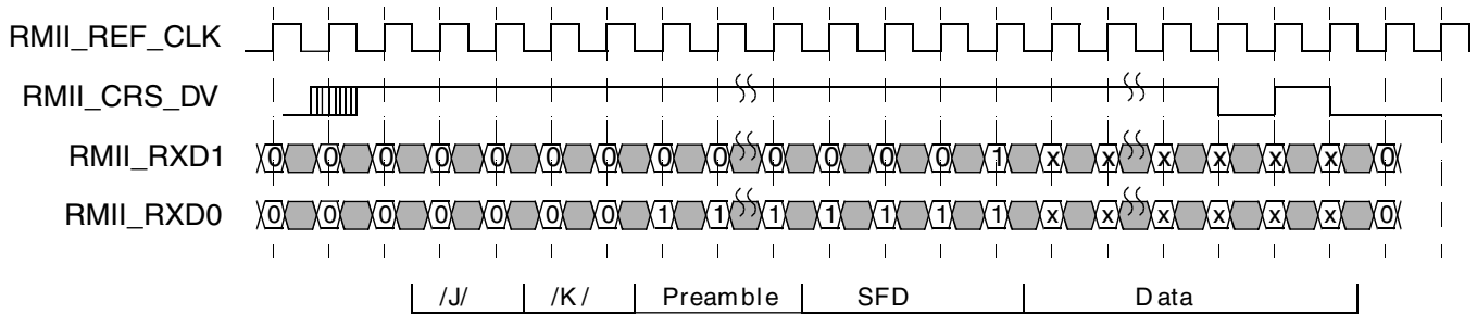
Figure 57-19. RMIi receive operation
