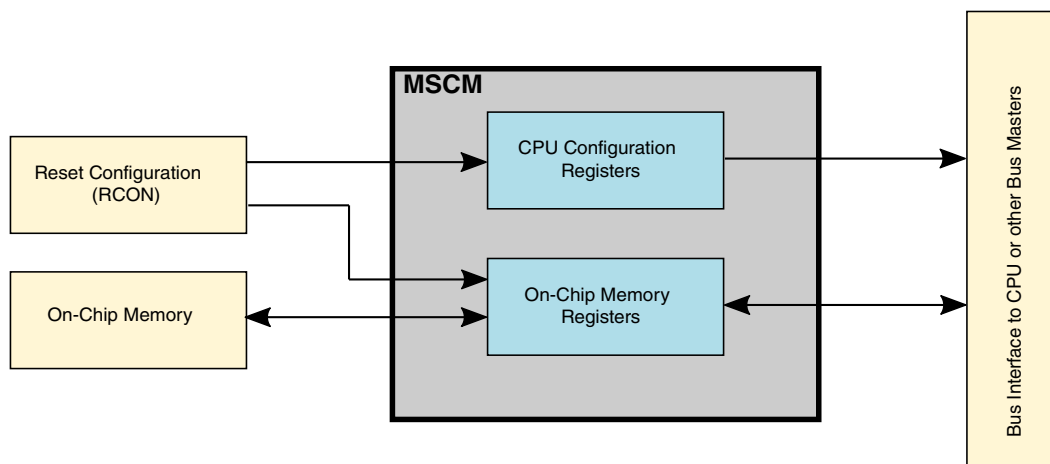
Figure 34-1. MSCM Block Diagram
