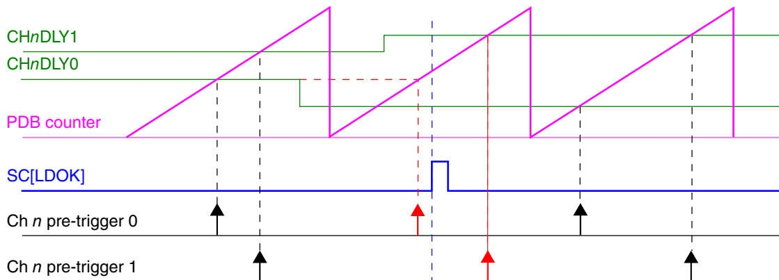
Figure 46-10. Registers update with SC[LDMOD] = 00
