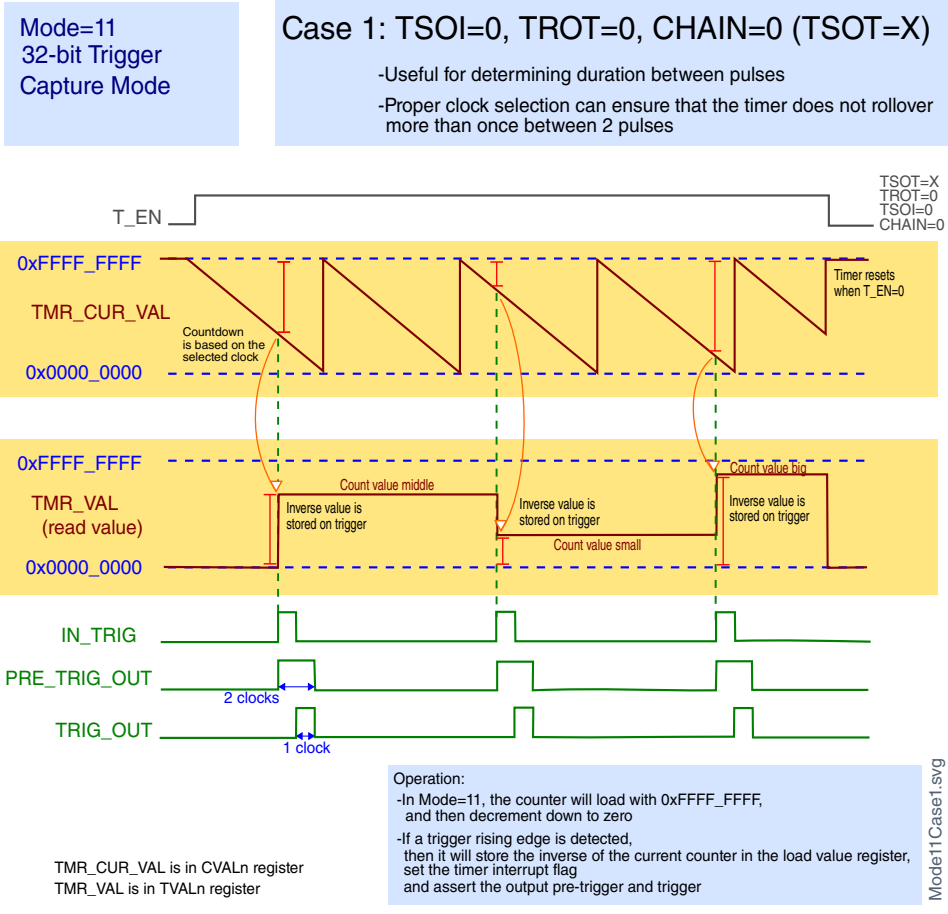
Figure 48-16. Case 1: TSOT = X, TROT = 0, TSOI = 0, CHAIN = 0
