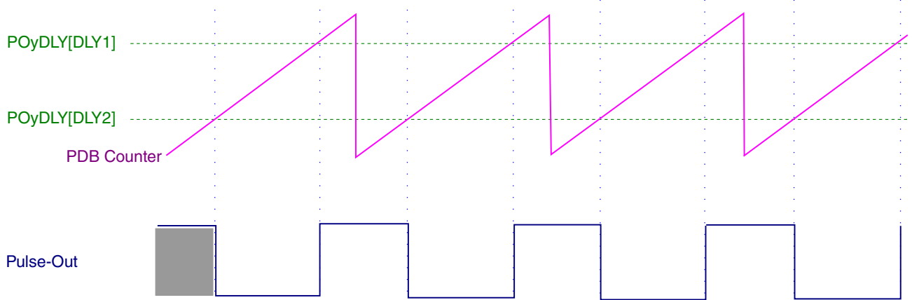
Figure 46-9. How Pulse Out is generated
