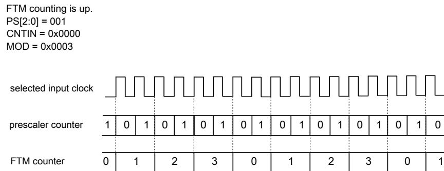
Figure 47-7. Example of the prescaler counter
