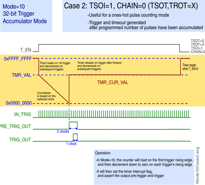
Figure 48-15. Case 2: TSOT = X, TROT = X, TSOI = 1, CHAIN = 0
