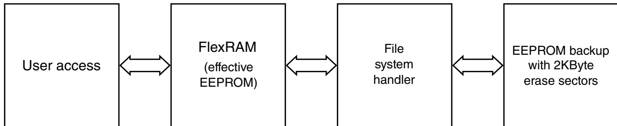
Figure 37-5. Top-level emulated EEPROM architecture
