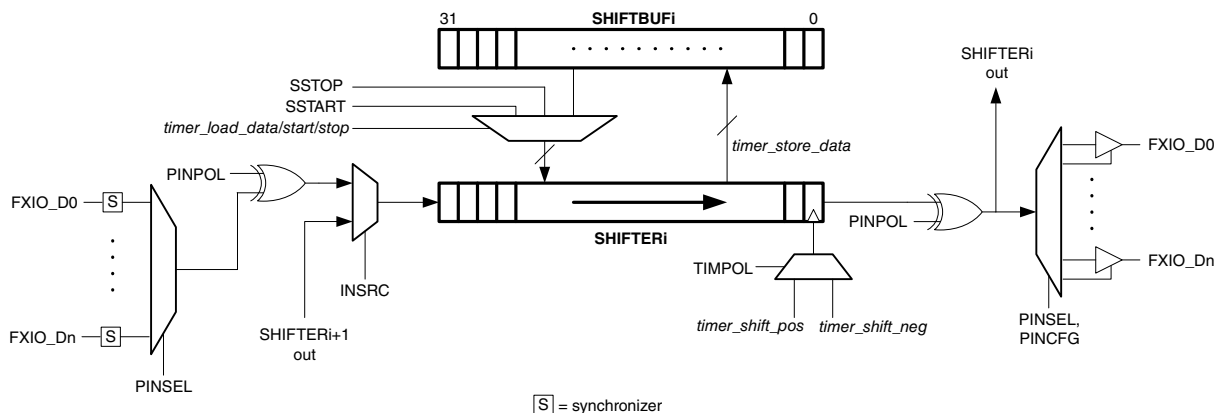
Figure 54-2. Shifter Microarchitecture
