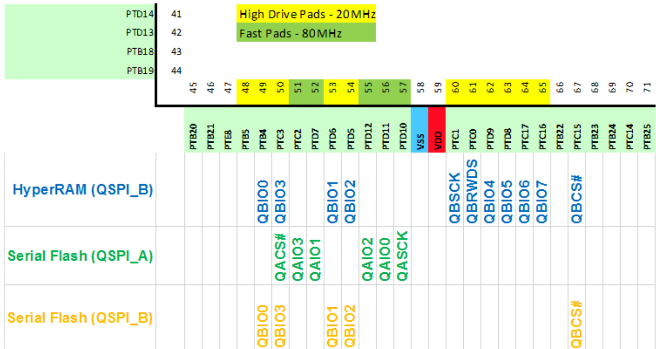
Figure 38-1. External memory options
