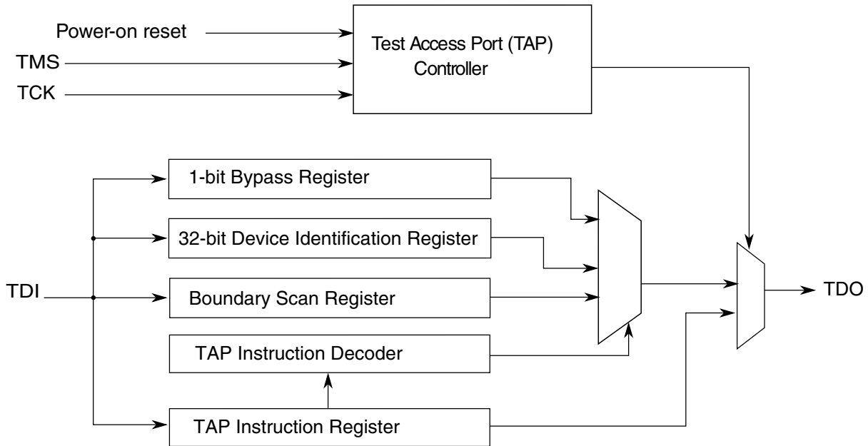
Figure 59-1. JTAG (IEEE 1149.1) block diagram
