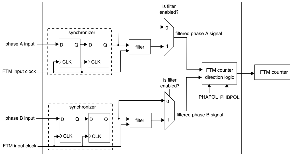
Figure 47-101. Diagram for Quadrature Decoder when FLTIPS[3:0] = 0
