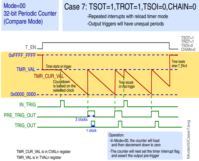
Figure 48-11. Case 7: TSOT = 1, TROT = 1, TSOI = 0, CHAIN = 0
