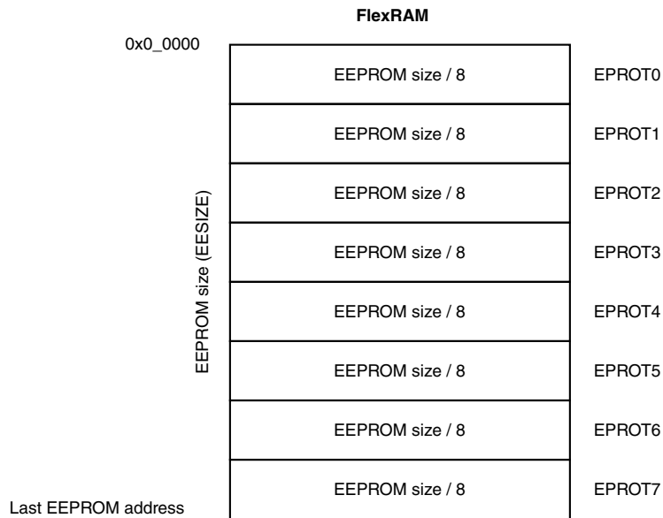
Figure 37-4. EEPROM protection
